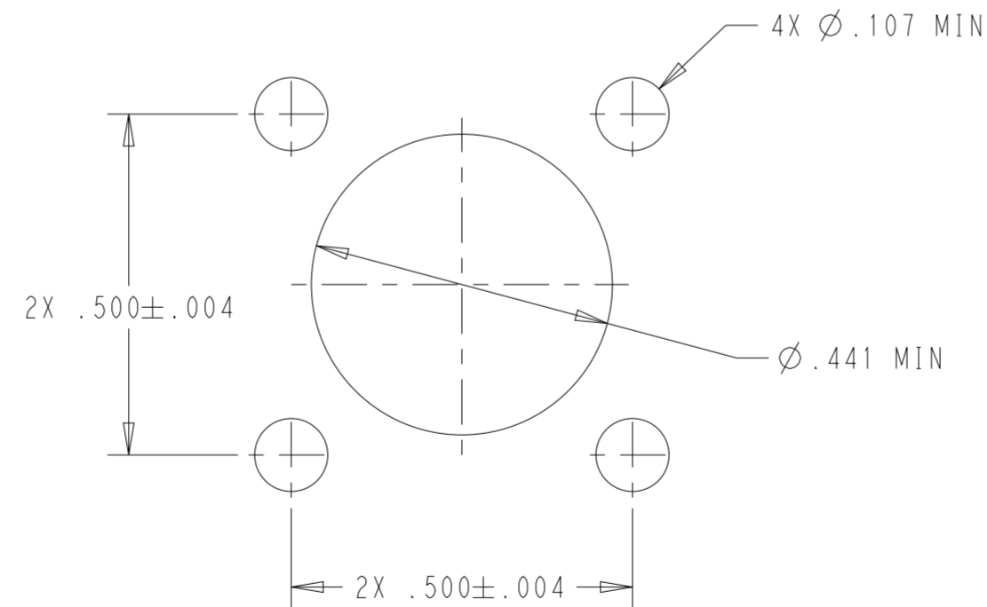
PANEL CUTOUT
