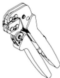
PRO-CRIMPER III Hand Tool Assembly 58560-1 (for 10-Position Modular Plugs) (408-4093)
