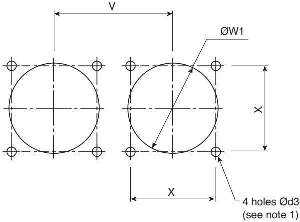
Rear Mounting Receptacle
